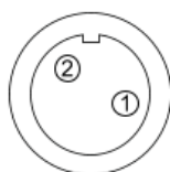
2 pins Binder 712 female connector (external view)
