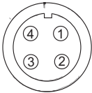
4 pin female connector - pinout external view
