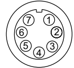
7 PINS binder 712 female connector (external view)
