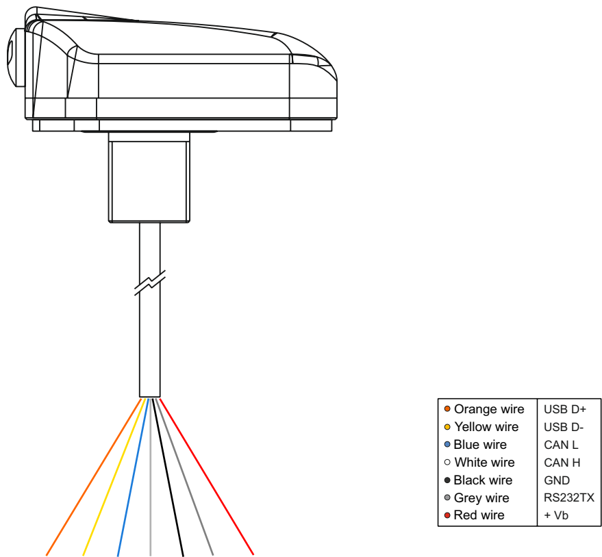
GPS09c Open and Pro Open, Roof version - Free wires
