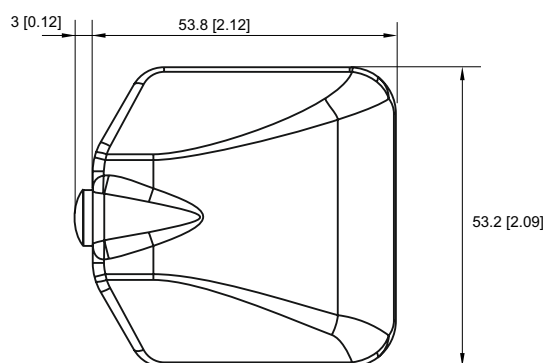
GPS09c Open and Pro Open, Roof version - free wires
