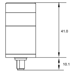
SMARTYCAM 3 GP BULLET CAM 67°- 84°
